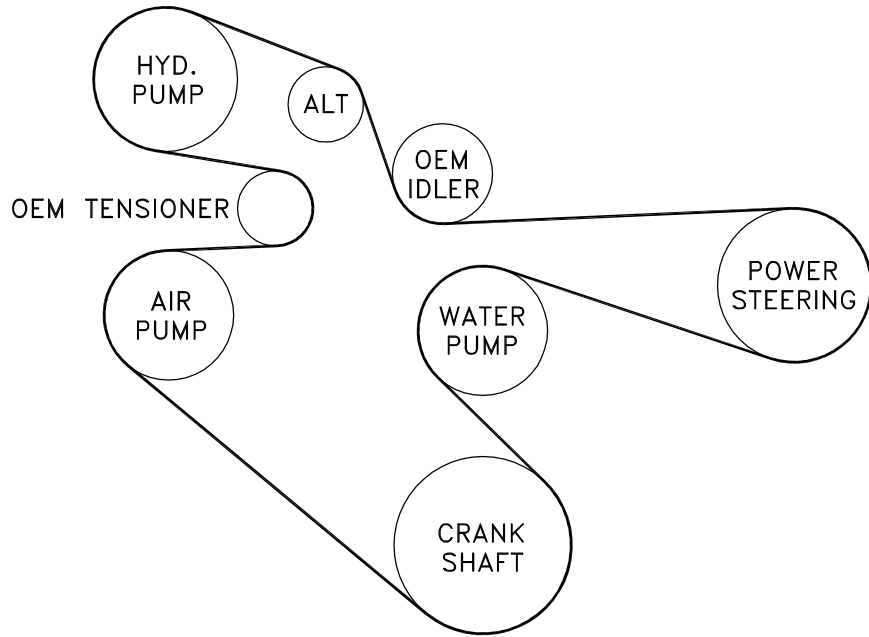
BELT DIAGRAM
