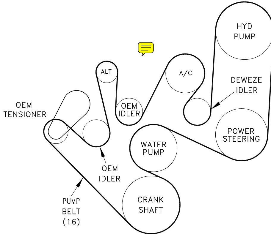
FIG. 1 BELT DIAGRAM
